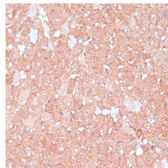
Immunohistochemistry of paraffin-embedded rat heart using ARHGAP4 antibody (STJ11100294) at dilution of 1:100 (40x lens).
