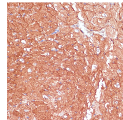
Immunohistochemistry of paraffin-embedded mouse heart using ARHGAP4 antibody (STJ11100294) at dilution of 1:100 (40x lens).
