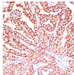
Immunohistochemistry of paraffin-embedded human thyroid cancer using ARHGAP4 antibody (STJ11100294) at dilution of 1:100 (40x lens).
