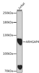
Western blot analysis of extracts of Jurkat cells, using ARHGAP4 rabbit polyclonal antibody (STJ11100294) at 1:1000 dilution. Secondary antibody: HRP Goat Anti-rabbit IgG (H+L) at 1:10000 dilution. Lysates/proteins: 25µg per lane. Blocking buffer: 3% nonfat dry milk in TBST. Detection: ECL Basic Kit. Exposure time: 90s.
