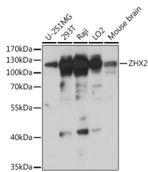
Western blot analysis of extracts of various cell lines, using ZHX2 antibody (STJ11100192) at 1:1000 dilution. Secondary antibody: HRP-Goat Anti-rabbit IgG (H+L) at 1:10000 dilution. Lysates/proteins: 25ug per lane. Blocking buffer: 3% nonfat dry milk in TBST. Detection: ECL Basic Kit. Exposure time: 10s.
