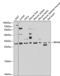
Western blot analysis of extracts of various cell lines, using BPGM antibody (STJ110190) at 1:1000 dilution. Secondary antibody: HRP Goat Anti-rabbit IgG (H+L) at 1:10000 dilution. Lysates/proteins: 25µg per lane. Blocking buffer: 3% nonfat dry milk in TBST. Detection: ECL Basic Kit. Exposure time: 30s.
