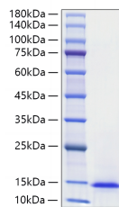
Recombinant Mouse Midkine Protein was determined by SDS-PAGE with Coomassie Blue, showing a band at 10-15 kD.
