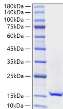
Recombinant Mouse Galectin-1/LGALS1 Protein was determined by SDS-PAGE with Coomassie Blue, showing a band at 15-20 kDa.
