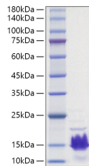
Recombinant Human Parathormone/PTH Protein was determined by SDS-PAGE with Coomassie Blue, showing a band at 14-18 kDa.
