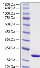
Recombinant Mouse PPIase A/PPIA Protein was determined by SDS-PAGE with Coomassie Blue, showing bands at 15-25 kDa.
