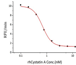
Recombinant Human OSM inhibits papain cleavage of a fluorogenic peptide substrate Z-FR-AMC. The IC50 value is <0.7 nM.
