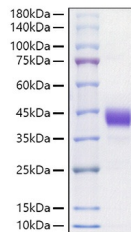
Recombinant Mouse CD52 Protein was determined by SDS-PAGE with Coomassie Blue, showing a band at 40-45 kDa.
