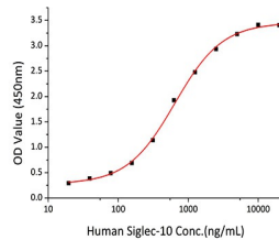
Immobilized Mouse CD52 at 10 Mu g/mL (100 Mu L/well) can bind Human Siglec-10 with a linear range of 0.3-642 ng/mL.
