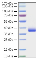
Recombinant SARS-CoV-2 Spike RBD (E484K) Protein was determined by SDS-PAGE with Coomassie Blue, showing a band at 36kDa.
