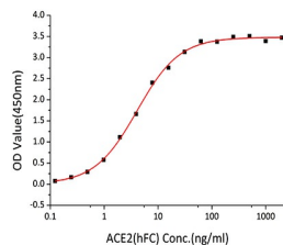
Immobilized SARS-CoV-2 Spike RBD (E484K) at 2 Mu g/mL (100 Mu L/well) can bind Human ACE2 (Catalog: STJP001274) with a linear range of 0.1-4.08 ng/mL.
