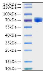
Recombinant Human EphA7/EHK-3 Protein was determined by SDS-PAGE with Coomassie Blue, showing a band at 70-80 kDa.
