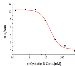
Recombinant Human CST5 inhibits papain cleavage of a fluorogenic peptide substrate Z-FR-AMC (Catalog # ES009). The IC50 value is <18 nM.
