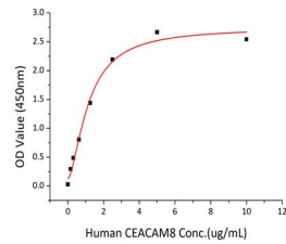
Immobilized Recombinant Human CEACAM1 at 5 Mu g/mL (100 Mu L/well) can bind Recombinant Human CEACAM8 with a linear range of 0.5-5 Mu g/mL.
