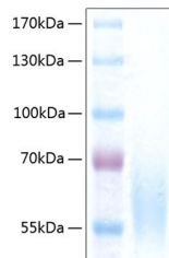
Recombinant Human CEACAM-1/CD66a Protein was determined by SDS-PAGE with Coomassie Blue, showing a band at 55-70 kDa.
