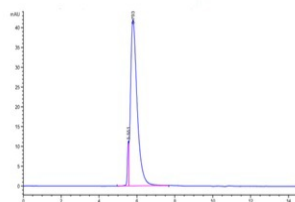
The purity of 2019-nCoV B.1.1.529 nucleocapsid is greater than 95% as determined by SEC-HPLC.
