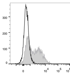
C57BL/6 murine splenocytes were stained with Anti-IgM antibody (STJA0001033) (filled gray histogram). Unstained splenocytes (empty black histogram) were used as control.
