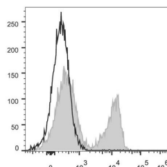
C57BL/6 murine splenocytes were stained with Anti-CD3 antibody (STJA0000187) (filled gray histogram). Unstained splenocytes (empty black histogram) were used as control.
