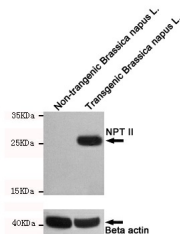
Western blot detection of NPTII in non-transgenic Brassica napus L. and transgenic Brassica napus L. cell lysates using NPTII mouse mAb (1:1000 diluted). Predicted band size: 29 kDa. Observed band size: 29 kDa.
