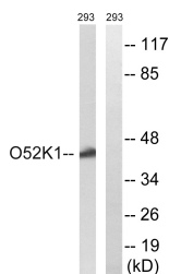
Western blot analysis of lysates from 293 cells, using OR52K1 Antibody. The lane on the right is blocked with the synthesized peptide.
