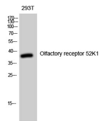
Western blot analysis of 293T cells using Olfactory receptor 52K1 Polyclonal Antibody diluted at 1/1000.
