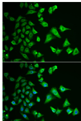
Immunofluorescence analysis of HeLa cells using DHRS2 antibody (STJ28529). Blue: DAPI for nuclear staining.
