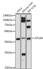
Western blot analysis of extracts of various cell lines, using ATG4A antibody (STJ22708) at 1:500 dilution. Secondary antibody: HRP Goat Anti-Rabbit IgG (H+L) (STJ3000896) at 1:10000 dilution. Lysates/proteins: 25 \mu g per lane. Blocking buffer: 3% nonfat dry milk in TBST. Detection: ECL Basic Kit. Exposure time: 180s.
