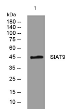
Western blot analysis of lysates from HpeG2 cells, primary antibody was diluted at 1:1000, 44°C over night
