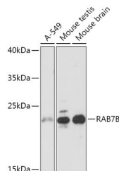
Western blot analysis of extracts of various cell lines, using RAB7B antibody (STJ119868) at 1:1000 dilution. Secondary antibody: HRP Goat Anti-rabbit IgG (H+L) at 1:10000 dilution. Lysates/proteins: 25 \mu g per lane. Blocking buffer: 3% nonfat dry milk in TBST. Detection: ECL Basic Kit. Exposure time: 3s.
