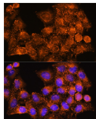
Immunofluorescence analysis of HeLa cells using RAB7B rabbit polyclonal antibody (STJ119868) at dilution of 1:100. Blue: DAPI for nuclear staining.
