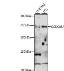
Western blot analysis of extracts of various cell lines, using CCDC88A antibody (STJ118572) at 1:1000 dilution. Secondary antibody: HRP Goat Anti-rabbit IgG (H+L) (STJS000856) at 1:10000 dilution. Lysates/proteins: 25 Mu g per lane. Blocking buffer: 3% non-fat dry milk in TBST. Detection: ECL Basic Kit. Exposure time: 90s.
