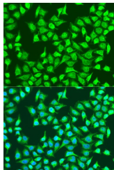
Immunofluorescence analysis of U2OS cells using SIRT4 antibody (STJ118245) at dilution of 1:100. Blue: DAPI for nuclear staining.
