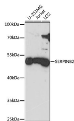
Western blot analysis of various lysates using SERPINB2 Rabbit polyclonal antibody (STJ117492) at 1:1000 dilution. Secondary antibody: HRP Goat Anti-Rabbit IgG (H+L) (STJ5000856) at 1:10000 dilution. Lysates/proteins: 25 µg per lane. Blocking buffer: 3% nonfat dry milk in TBST. Detection: ECL Basic Kit. Exposure time: 90s.
