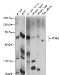
Western blot analysis of various lysates using PTPRG Rabbit polyclonal antibody (STJ116466) at 1:1000 dilution. Secondary antibody: HRP Goat Anti-Rabbit IgG (H+L) (STJS000856) at 1:10000 dilution. Lysates/proteins: 25 µg per lane. Blocking buffer: 3% nonfat dry milk in TBST. Detection: ECL Basic Kit. Exposure time: 90s.
