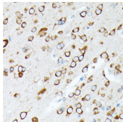
Immunohistochemistry analysis of RPL7 in paraffin-embedded rat brain using RPL7 Rabbit polyclonal antibody (STJ116287) at dilution of 1:100 (40x lens). Perform microwave antigen retrieval with 10 mM PBS buffer pH 7.2 before commencing with immunohistochemistry staining protocol.
