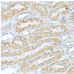
Immunohistochemistry analysis of RPL7 in paraffin-embedded mouse kidney using RPL7 Rabbit polyclonal antibody (STJ116287) at dilution of 1:100 (40x lens). Perform microwave antigen retrieval with 10 mM PBS buffer pH 7.2 before commencing with immunohistochemistry staining protocol.
