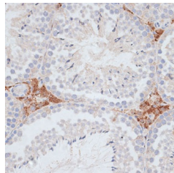
Immunohistochemistry analysis of KIFC1 in paraffin-embedded mouse testis using KIFC1 Rabbit polyclonal antibody (STJ116198) at dilution of 1:100 (40x lens). Perform microwave antigen retrieval with 10 mM PBS buffer pH 7.2 before commencing with immunohistochemistry staining protocol.
