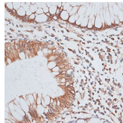
Immunohistochemistry analysis of KIFC1 in paraffin-embedded human colon carcinoma using KIFC1 Rabbit polyclonal antibody (STJ116198) at dilution of 1:100 (40x lens). Perform microwave antigen retrieval with 10 mM PBS buffer pH 7.2 before commencing with immunohistochemistry staining protocol.
