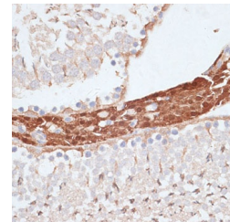
Immunohistochemistry analysis of KIFC1 in paraffin-embedded rat testis using KIFC1 Rabbit polyclonal antibody (STJ116198) at dilution of 1:100 (40x lens). Perform microwave antigen retrieval with 10 mM PBS buffer pH 7.2 before commencing with immunohistochemistry staining protocol.
