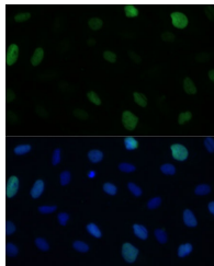
Immunofluorescence analysis of U-2 OS cells using KIFC1 Rabbit polyclonal antibody (STJ116198) at dilution of 1:100 (40x lens). Secondary antibody: Cy3 Goat Anti-Rabbit IgG (H+L) at 1:500 dilution. Blue: DAPI for nuclear staining.
