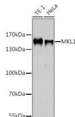
Western blot analysis of extracts of various cell lines, using MKL1 antibody (STJ116144) at 1:1000 dilution. Secondary antibody: HRP Goat Anti-Rabbit IgG (H+L) (STJ3000896) at 1:10000 dilution. Lysates/proteins: 25 \mu g per lane. Blocking buffer: 3% nonfat dry milk in TBST. Detection: ECL Basic Kit. Exposure time: 30s.
