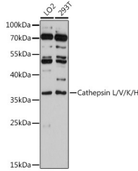
Western blot analysis of various lysates using Cathepsin L/V/K/H Rabbit polyclonal antibody (STJ113965) at 1:3000 dilution. Secondary antibody: HRP Goat Anti-Rabbit IgG (H+L) (STJS000856) at 1:10000 dilution. Lysates/proteins: 25 Mu g per lane. Blocking buffer: 3% nonfat dry milk in TBST. Detection: ECL Basic Kit. Exposure time: 90s.
