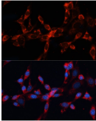
Immunofluorescence analysis of NIH/3T3 cells using Cathepsin L/V/K/H Rabbit polyclonal antibody (STJ113965) at dilution of 1:100. Secondary antibody: Cy3 Goat Anti-Rabbit IgG (H+L) at 1:500 dilution. Blue: DAPI for nuclear staining.
