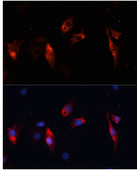
Immunofluorescence analysis of C6 cells using Cathepsin L/V/K/H Rabbit polyclonal antibody (STJ113965) at dilution of 1:100. Secondary antibody: Cy3 Goat Anti-Rabbit IgG (H+L) at 1:500 dilution. Blue: DAPI for nuclear staining.
