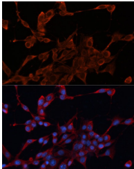
Immunofluorescence analysis of NIH/3T3 cells using [KO Validated] DNAJA1 Rabbit polyclonal antibody (STJ113207) at dilution of 1:100. Secondary antibody: Cy3 Goat Anti-Rabbit IgG (H+L) at 1:500 dilution. Blue: DAPI for nuclear staining.
