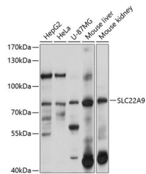
Western blot analysis of extracts of various cell lines, using SLC22A9 antibody (STJ112465) at 1:1000 dilution. Secondary antibody: HRP Goat Anti-rabbit IgG (H+L) at 1:10000 dilution. Lysates/proteins: 25µg per lane. Blocking buffer: 3% nonfat dry milk in TBST. Detection: ECL Basic Kit. Exposure time: 10s.
