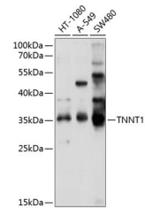
Western blot analysis of extracts of various cell lines, using TNNT1 antibody (STJ112391) at 1:1000 dilution. Secondary antibody: HRP Goat Anti-Rabbit IgG (H+L) (STJS000856) at 1:10000 dilution. Lysates/proteins: 25 Mu g per lane. Blocking buffer: 3% nonfat dry milk in TBST. Detection: ECL Basic Kit. Exposure time: 15s.
