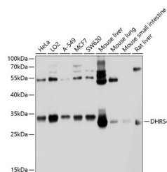
Western blot analysis of extracts of various cell lines, using DHRS4 antibody (STJ112323) at 1:1000 dilution. Secondary antibody: HRP Goat Anti-Rabbit IgG (H+L) (STJ5000856) at 1:10000 dilution. Lysates/proteins: 25 µg per lane. Blocking buffer: 3% nonfat dry milk in TBST. Detection: ECL Basic Kit. Exposure time: 1s.
