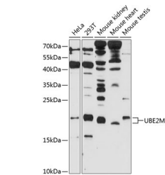
Western blot analysis of extracts of various cell lines, using UBE2M antibody (STJ111518) at 1:1000 dilution. Secondary antibody: HRP Goat Anti-rabbit IgG (H+L) at 1:10000 dilution. Lysates/proteins: 25ug per lane. Blocking buffer: 3% nonfat dry milk in TBST. Detection: ECL Basic Kit. Exposure time: 90s.
