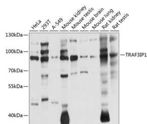
Western blot analysis of extracts of various cell lines, using TRAF3IP1 antibody (STJ111513) at 1:1000 dilution. Secondary antibody: HRP Goat Anti-rabbit IgG (H+L) at 1:10000 dilution. Lysates/proteins: 25 µg per lane. Blocking buffer: 3% nonfat dry milk in TBST. Detection: ECL Basic Kit. Exposure time: 3s.
