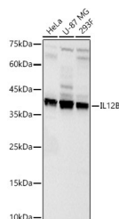
Western blot analysis of various lysates, using IL12B Rabbit polyclonal antibody (STJ11104995) at 1:800 dilution. Secondary antibody: HRP Goat Anti-Rabbit IgG (H+L) (STJS000856) at 1:10000 dilution. Lysates/proteins: 25µg per lane. Blocking buffer: 3% nonfat dry milk in TBST. Detection: ECL Basic Kit. Exposure time: 5s.
