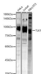
Western blot analysis of extracts of various cell lines, using TLK1 antibody (STJ11104634) at 1:1000 dilution. Secondary antibody: HRP Goat Anti-Rabbit IgG (H+L) (STJS000856) at 1:10000 dilution. Lysates/proteins: 25 Mu g per lane. Blocking buffer: 3% nonfat dry milk in TBST. Detection: ECL Enhanced Kit. Exposure time: 60s.
