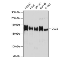
Western blot analysis of various lysates using DSG2 Rabbit polyclonal antibody (STJ11104316) at 1:1000 dilution. Secondary antibody: HRP Goat Anti-Rabbit IgG (H+L) (STJS000856) at 1:10000 dilution. Lysates/proteins: 25 µg per lane. Blocking buffer: 3% nonfat dry milk in TBST. Detection: ECL Basic Kit. Exposure time: 10s.
