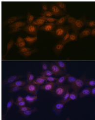
Immunofluorescence analysis of NIH-3T3 cells using WAPL Rabbit monoclonal antibody (STJ11103590) at dilution of 1:100 (40x lens). Blue: DAPI for nuclear staining.
