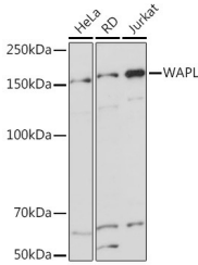
Western blot analysis of extracts of various cell lines, using WAPL Rabbit monoclonal antibody (STJ11103590) at 1:1000 dilution. Secondary antibody: HRP Goat Anti-Rabbit IgG (H+L) (STJS000856) at 1:10000 dilution. Lysates/proteins: 25 Mu g per lane. Blocking buffer: 3% nonfat dry milk in TBST. Detection: ECL Basic Kit. Exposure time: 1s.
