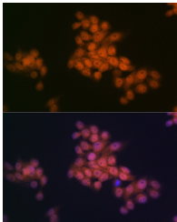
Immunofluorescence analysis of HeLa cells using WAPL Rabbit monoclonal antibody (STJ11103590) at dilution of 1:100 (40x lens). Blue: DAPI for nuclear staining.
