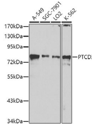
Western blot analysis of extracts of various cell lines, using PTCD3 antibody (STJ110795) at 1:1000 dilution. Secondary antibody: HRP Goat Anti-Rabbit IgG (H+L) (STJ5000856) at 1:10000 dilution. Lysates/proteins: 25 Mu g per lane. Blocking buffer: 3% nonfat dry milk in TBST. Detection: ECL Basic Kit. Exposure time: 90s.
